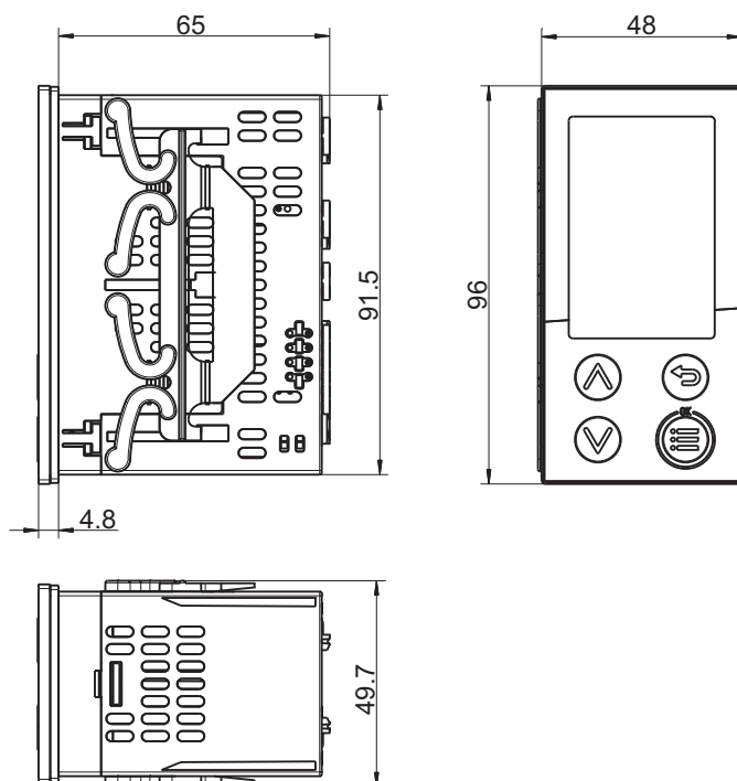
Typ 701512 (Format 108H: 48 mm × 96 mm)
